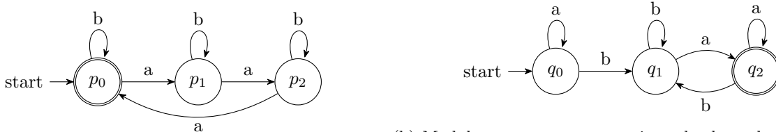
(a) Module to compute |w|_b \equiv |w| \pmod 3 . States q \in Q_a States p \in Q_b (b) Module to compute w contains sub. ba and ends in a .
